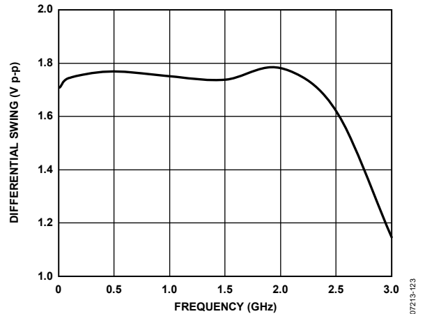
Figure 21. LVPECL Differential Voltage Swing vs. Frequency
